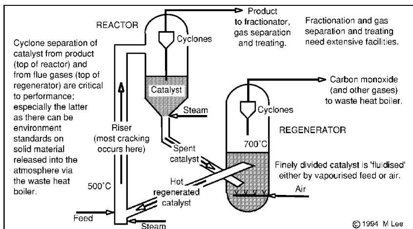
Figure 2.8 Catalytic cracking
