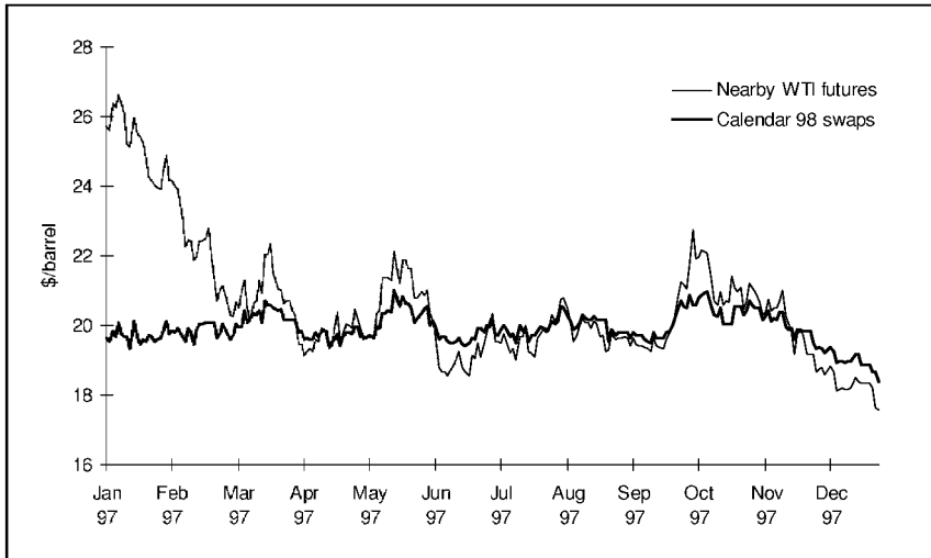
Figure 10.1 Nearby WTI futures and calendar 98 swaps prices
