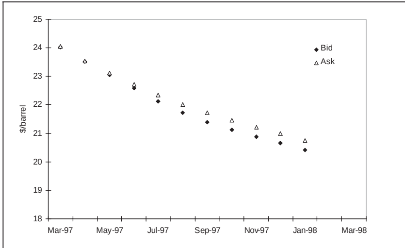
Figure 18.6 Bid-ask spread for WTI futures, 27 January 1997
