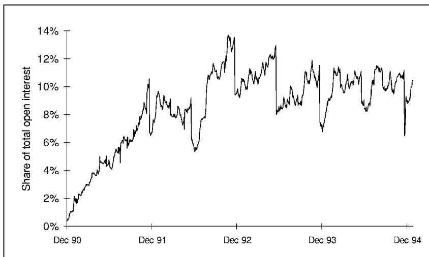
Figure 11.3 Share of WTI open interest 19 to 36 months ahead
