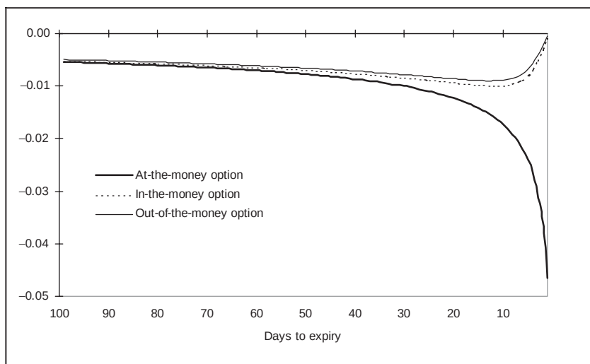
Figure 18.17 Changing value of theta for a call option
