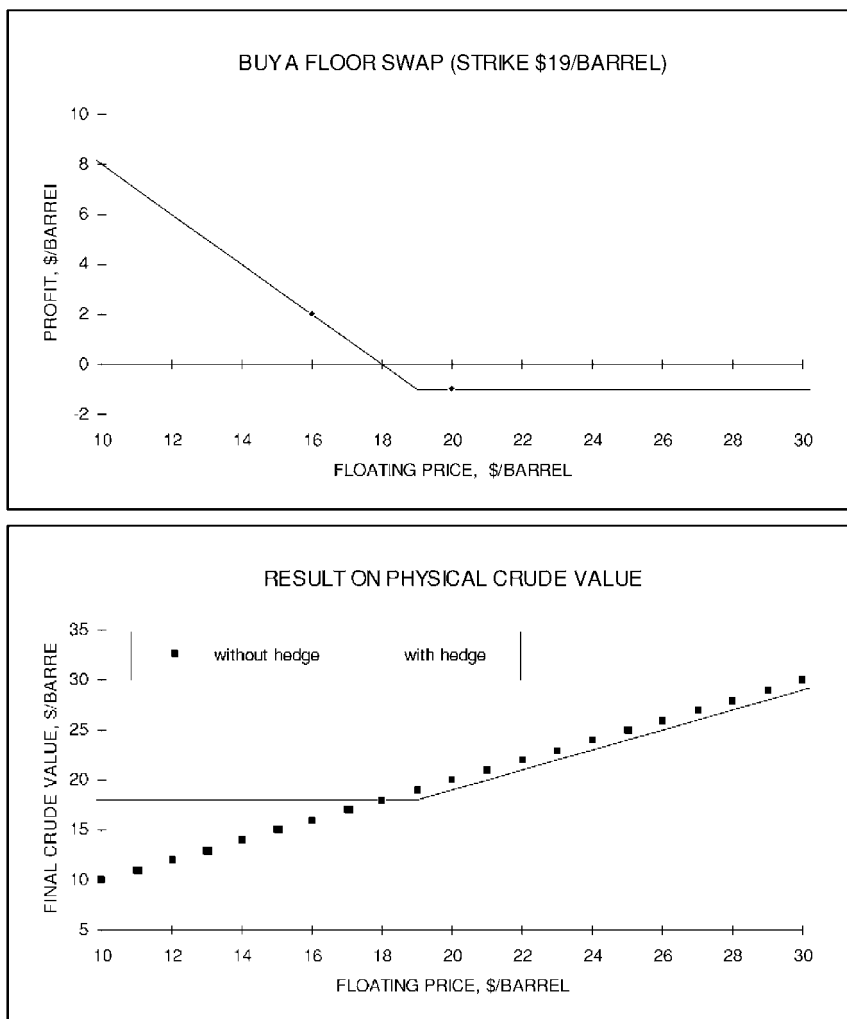
Figure 11.13 Purchase of a floor swap
