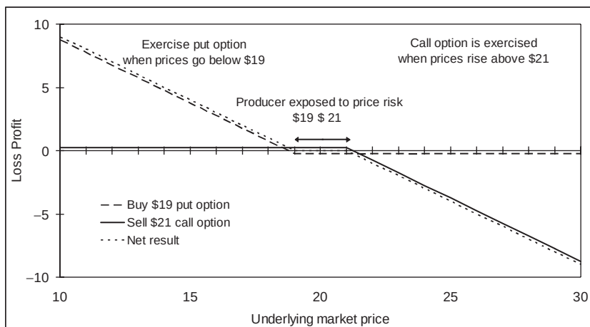
Figure 9.11 Hedging crude oil sales, zero cost collar
