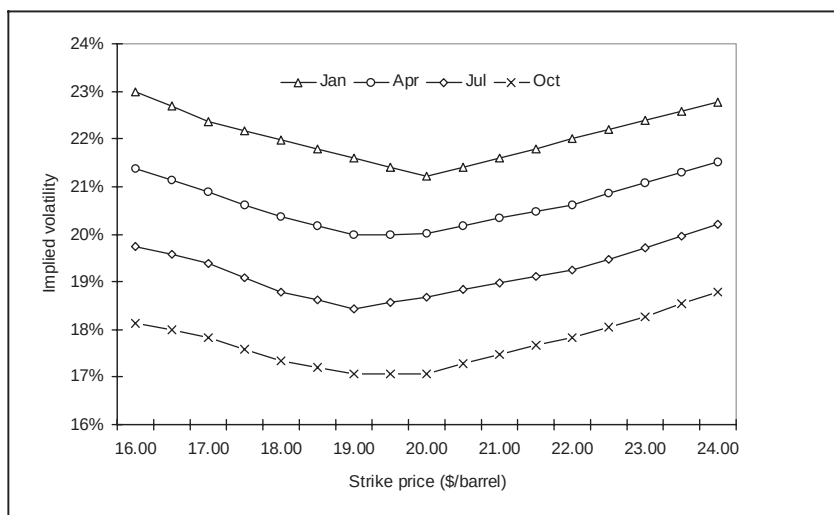
Figure 18.5 Volatility smiles, WTI options
