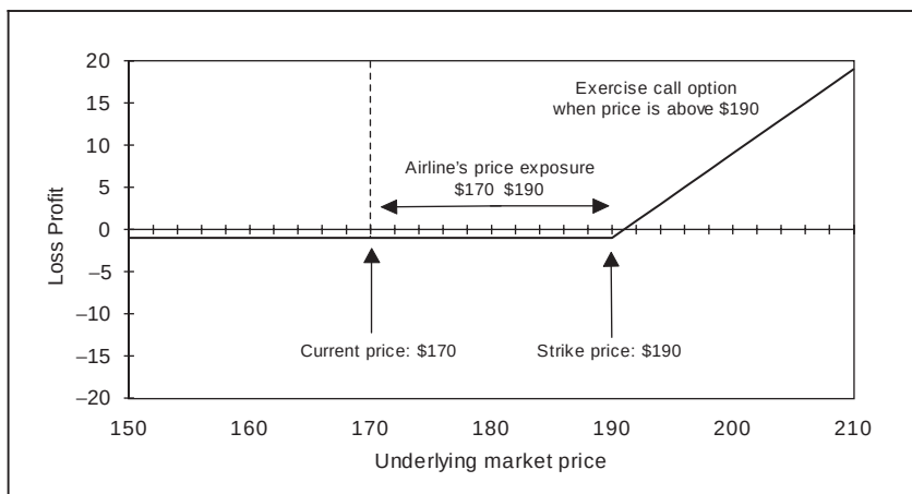
Figure 9.12 Hedging fuel purchases, buy a call option
