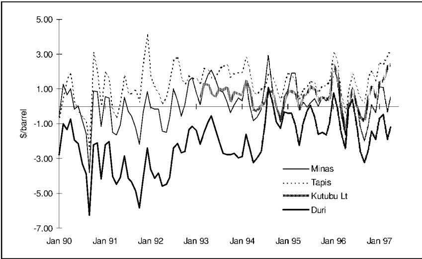
Figure 4.11 Asia Pacific crudes minus dated Brent
