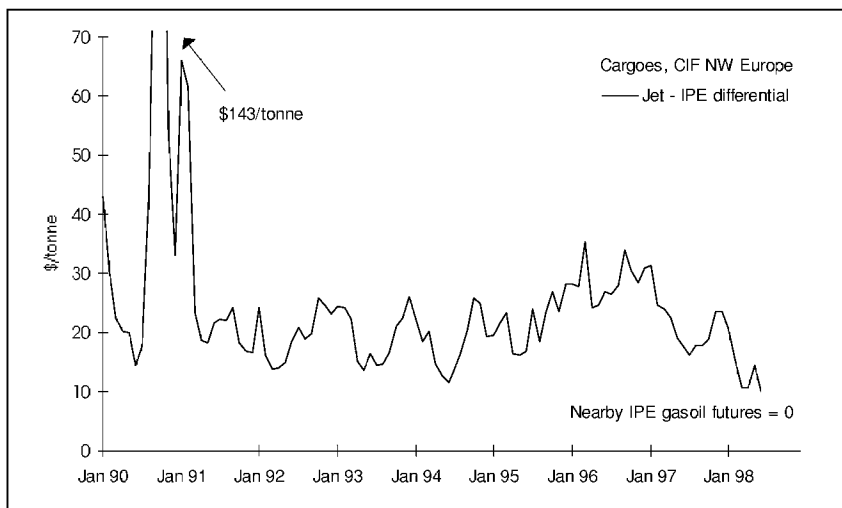
Figure 5.4 Jet kerosine minus nearby IPE gasoil futures prices
