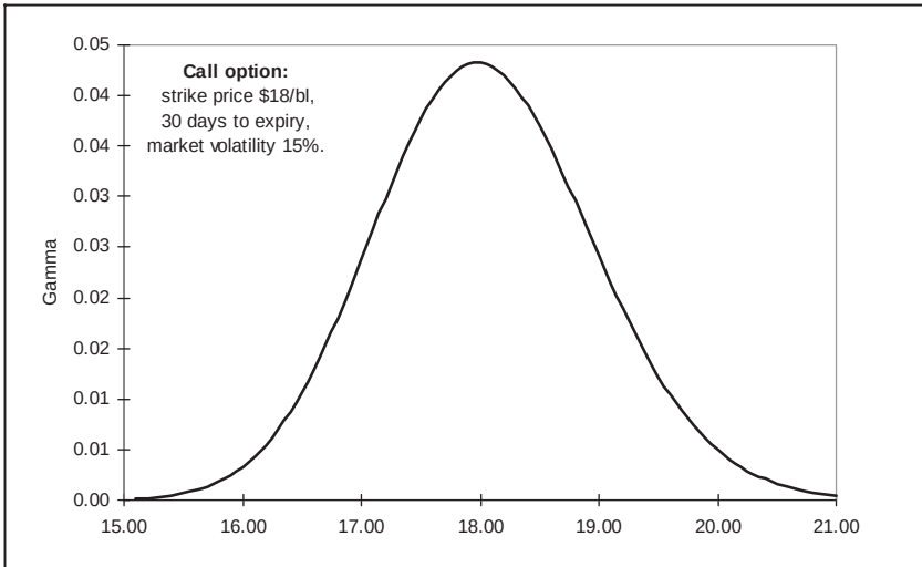
Figure 18.16 Changing value of gamma for a call option
