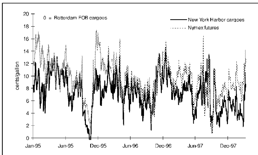
Figure 3.4 Unleaded gasoline, New York minus Rotterdam
