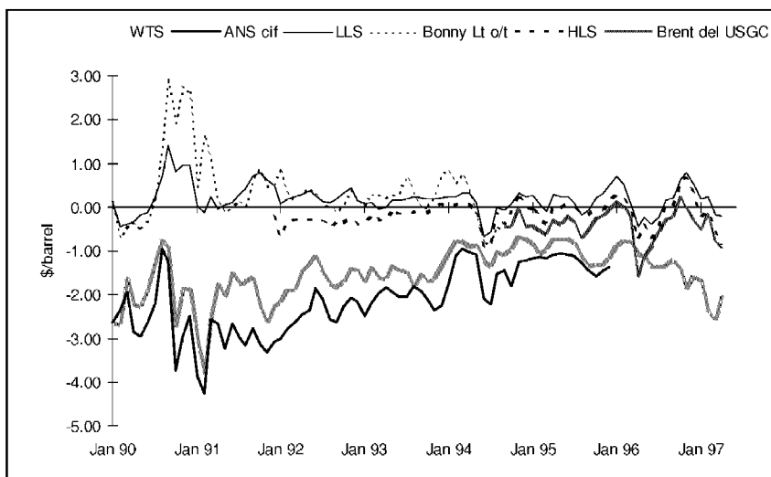
Figure 4.8 US Gulf coast crudes minus WTI Cushing
