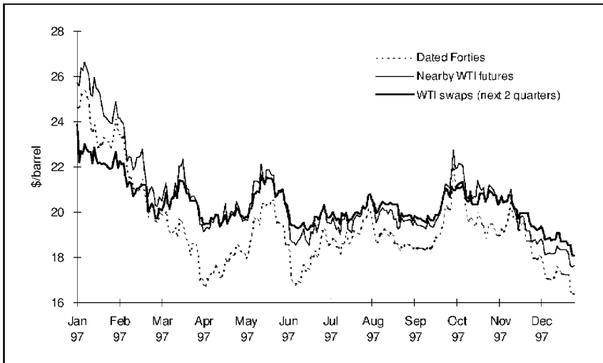
Figure 10.2 Dated Forties, WTI futures and swaps prices
