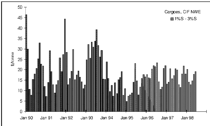
Figure 5.7 Low sulphur minus high sulphur fuel oil prices
