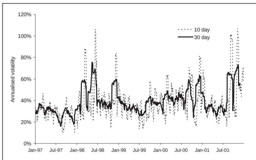
Figure 9.19 Historical price volatility, nearby WTI futures
