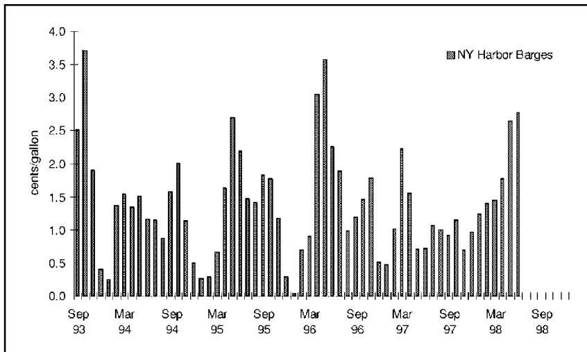
Figure 5.10 Distillate fuel oil: low sulphur diesel premium
