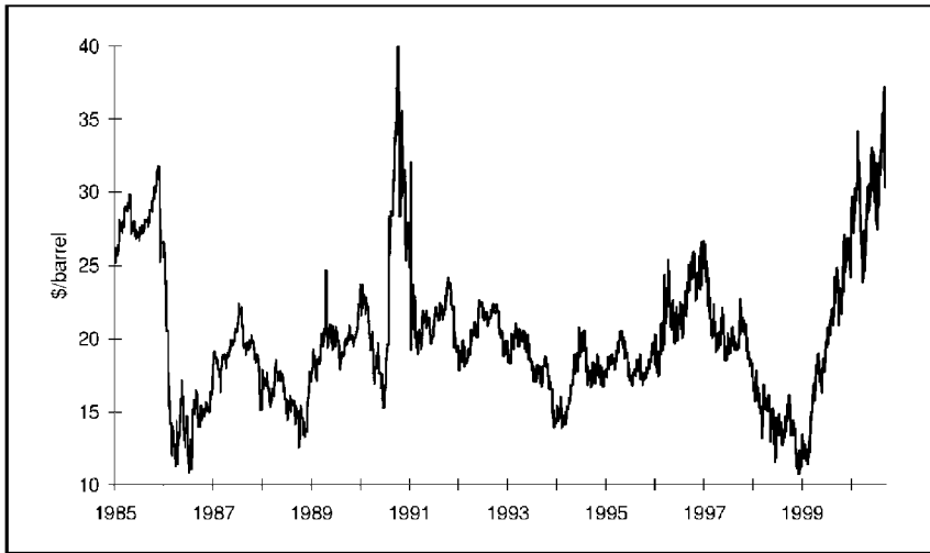
Figure 1.1 Crude oil prices, Nymex nearby WTI daily close
