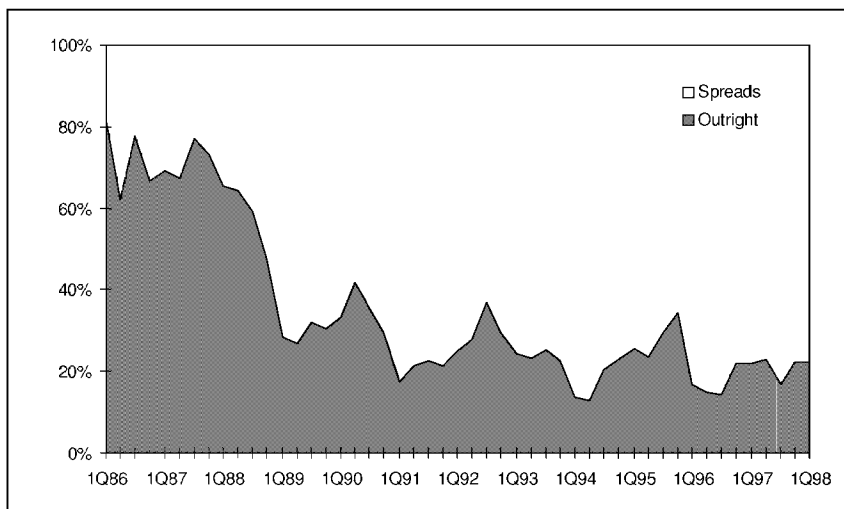
Figure 7.1 Share of outright deals in 15-day Brent market
