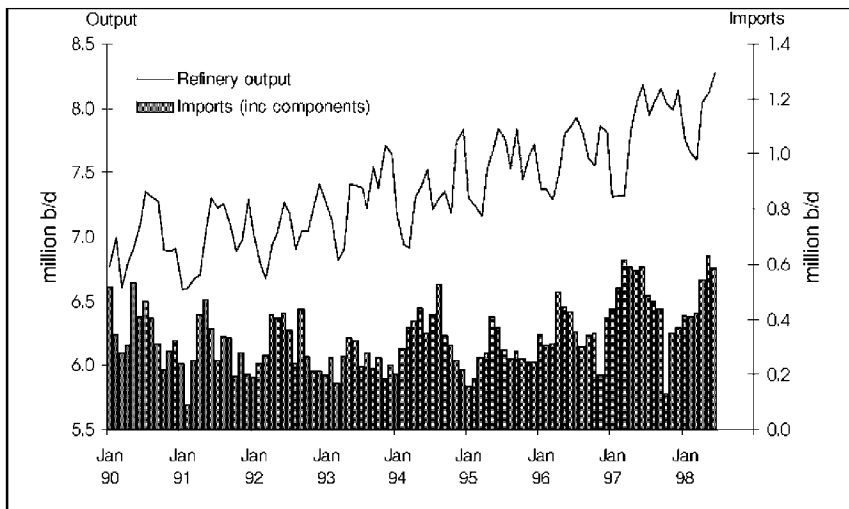
Figure 5.8 Gasoline: US refinery output and imports
