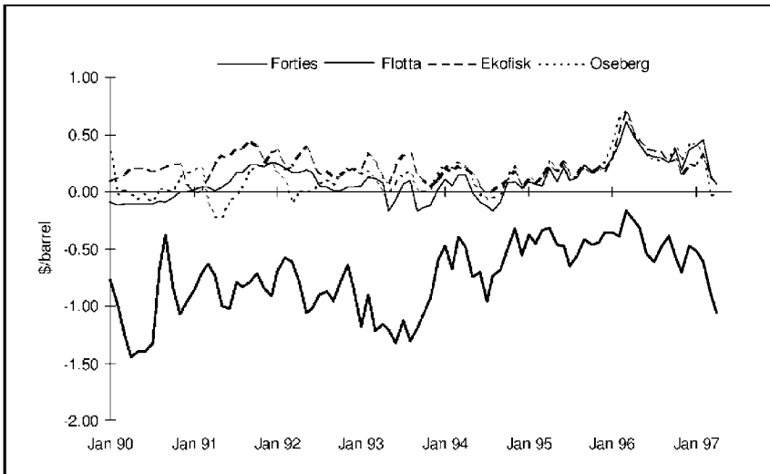
Figure 4.4 North Sea crudes minus dated Brent
