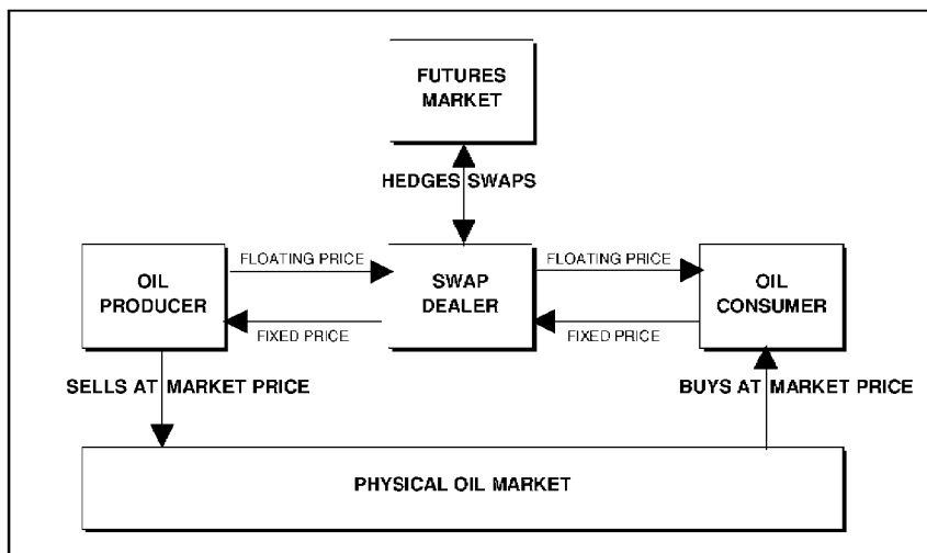
Figure 10.4 Structure of the swaps market
