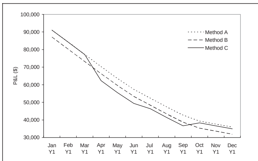
Figure 18.12 Tapis swap value using different price estimates
