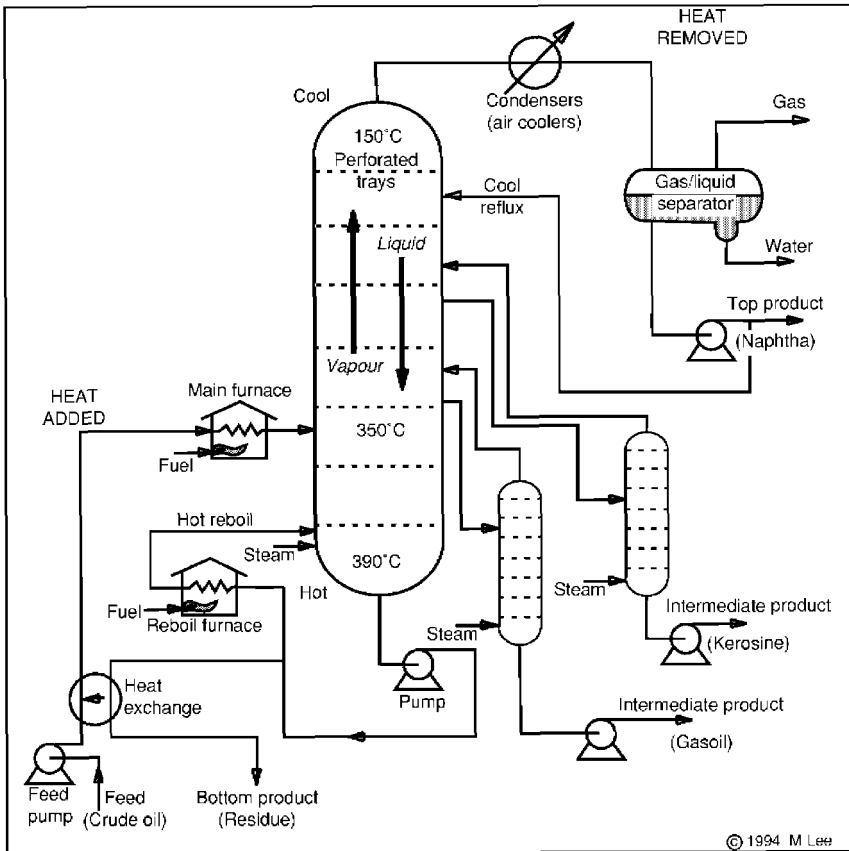
Figure 2.4 Fractional distillation
