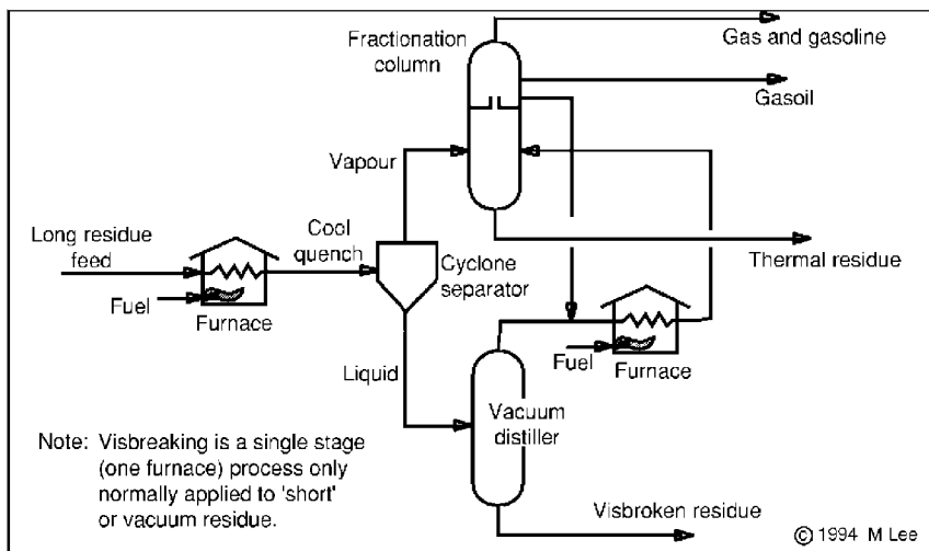
Figure 2.7 Thermal cracking (two-stage cracking)
