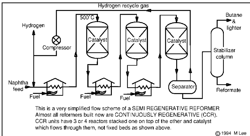
Figure 2.6 Catalytic reforming (platforming)
