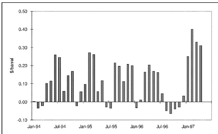
Figure 4.7 The Cushing Cushion, WTI Cushing–WTI Midland
