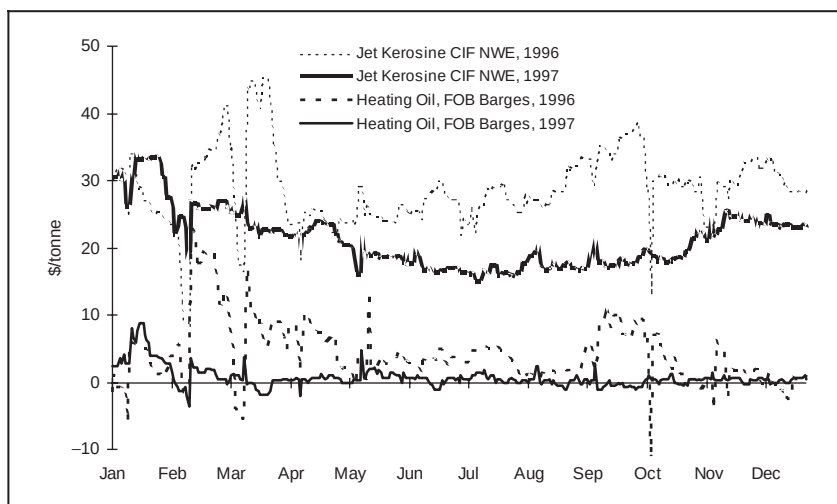
Figure 6.5 Basis risk against the IPE gasoil contract
