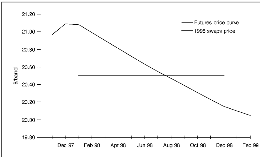
Figure 10.5 WTI forward curve and swaps price, 16 Oct 1997
