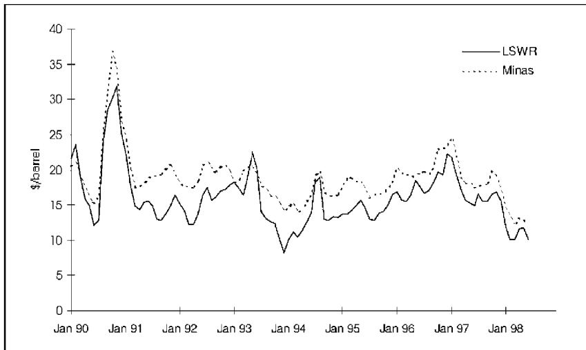
Figure 5.23 Low sulphur waxy residue & Minas crude prices
