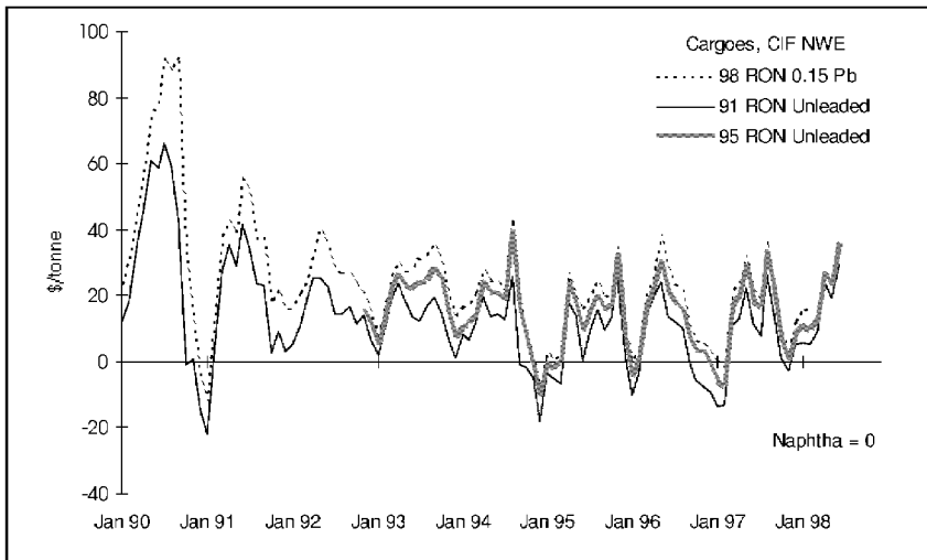
Figure 5.3 Gasoline minus naphtha prices
