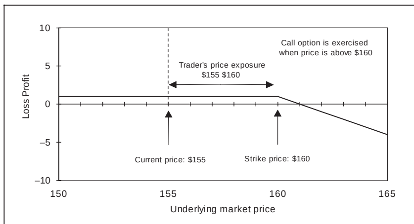
Figure 9.13 Reducing storage costs, sell a call option
