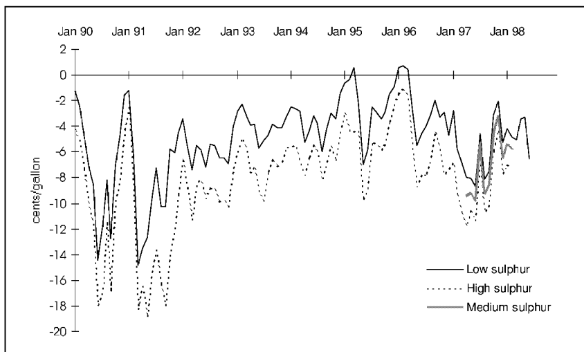
Figure 5.15 Vacuum gasoil: US Gulf coast cargo differentials
