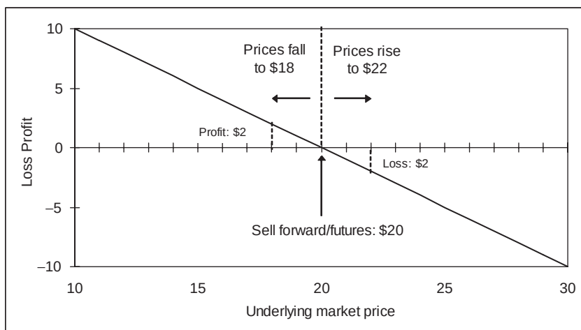
Figure 9.3 Selling a forward or futures contract
