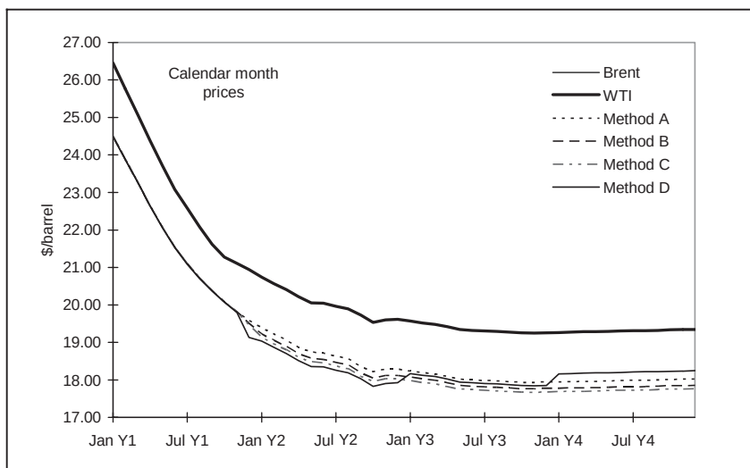
Figure 18.8 Estimated forward curves for Brent futures
