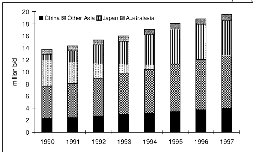
Figure 5.18 Asia Pacific oil demand growth, 1990-97
