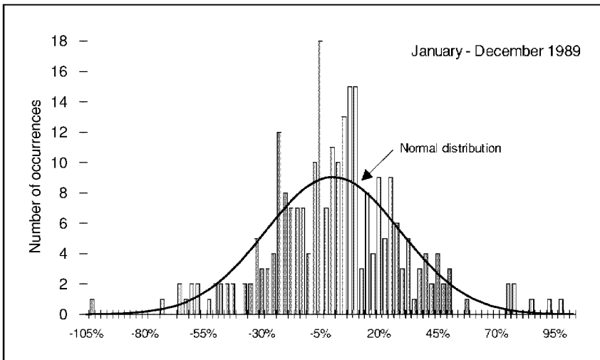
Figure 11.5 Distribution of daily returns for WTI-Brent spread
