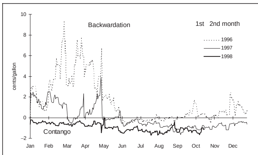
Figure 6.4 Nymex heating oil, contango and backwardation
