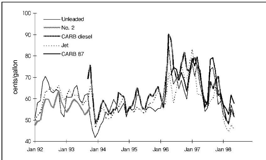
Figure 5.17 US west coast: Los Angeles pipeline prices
