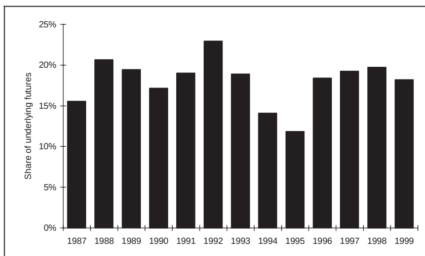
Figure 8.5 Nymex energy options as share of futures, 1987–99
