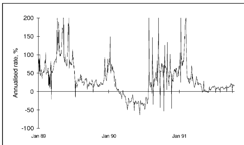
Figure 11.6 Convenience yield for nearby WTI futures
