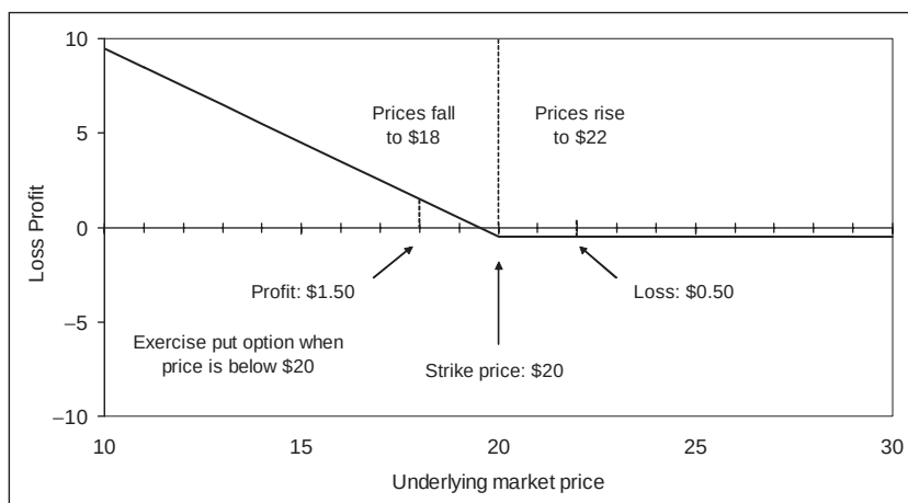
Figure 9.5 Payoff from buying a put option
