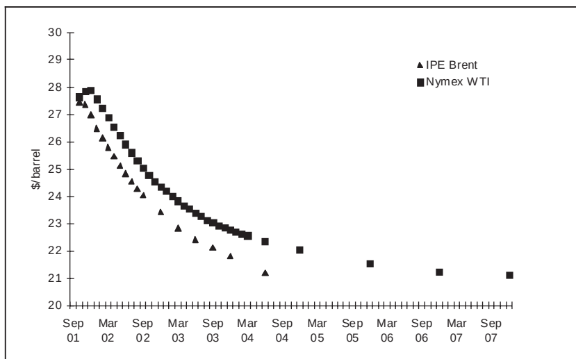
Figure 18.1 Forward price curves for WTI and Brent, 10/9/01
