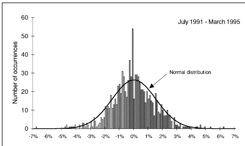
Figure 11.4 Distribution of daily returns for WTI first nearby
