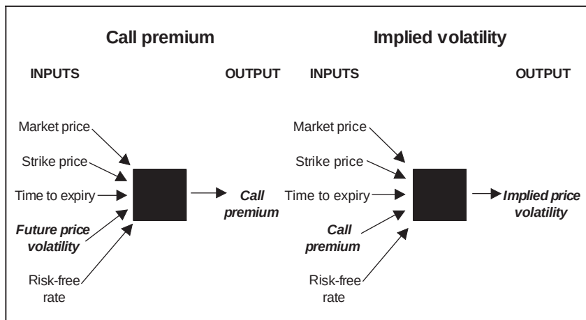
Figure 9.20 Using the Black-Scholes option pricing model
