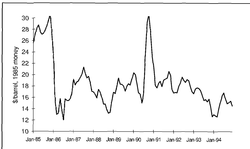
Figure 11.2 WTI price adjusted for inflation, 1985 dollars
