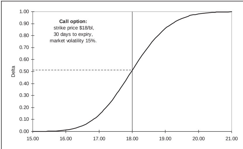
Figure 18.15 Changing value of delta for a call option
