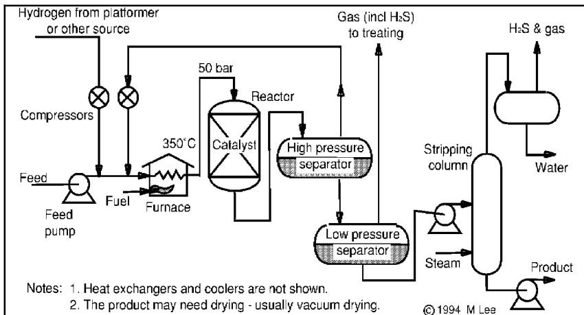
Figure 2.5 Hydrotreating (hydrodesulphurisation)
