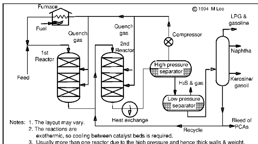
Figure 2.9 Hydrocracking
