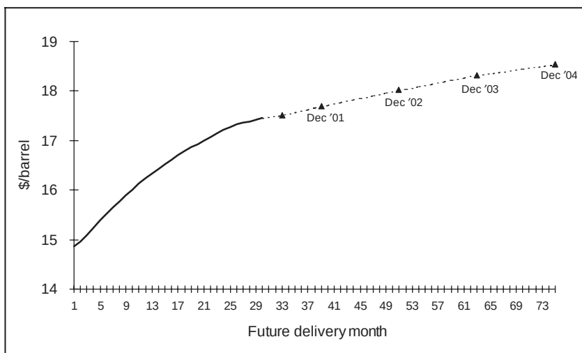
Figure 6.1 WTI futures price curve, 17 September 1998
