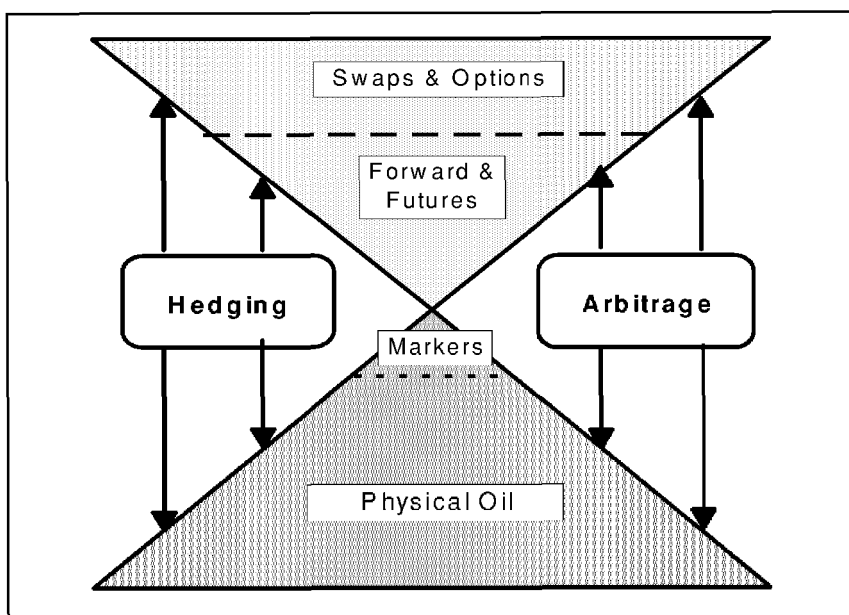
Figure 1.7 Structure of the oil market
