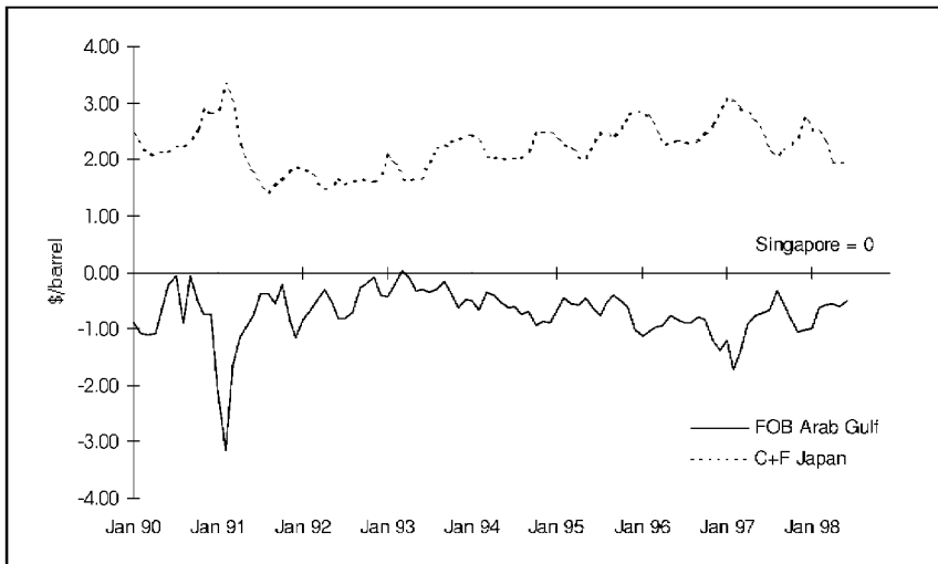
Figure 5.20 Naphtha: Arab Gulf & Japan minus Singapore prices
