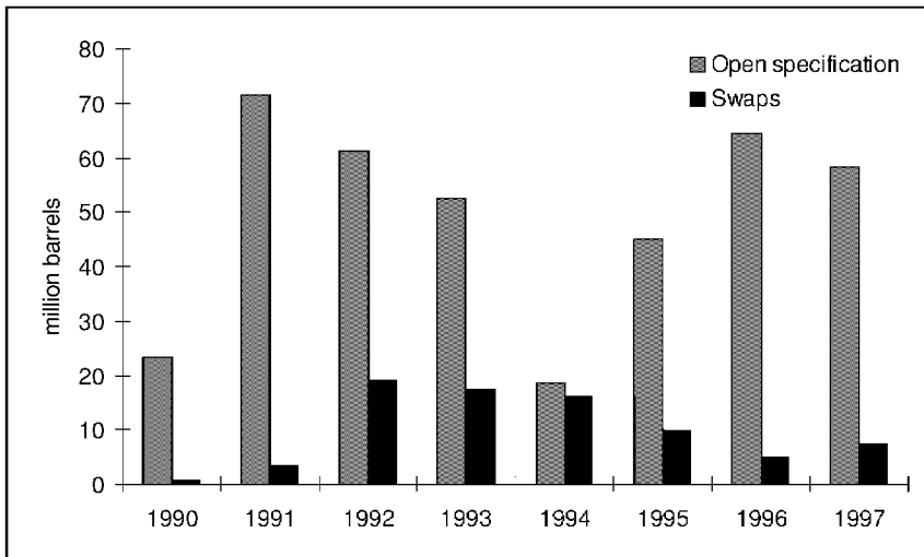
Figure 7.5 Trading volumes in the Asia Pacific naphtha market
