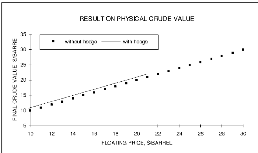
Figure 11.14 Sale of a ceiling swap
