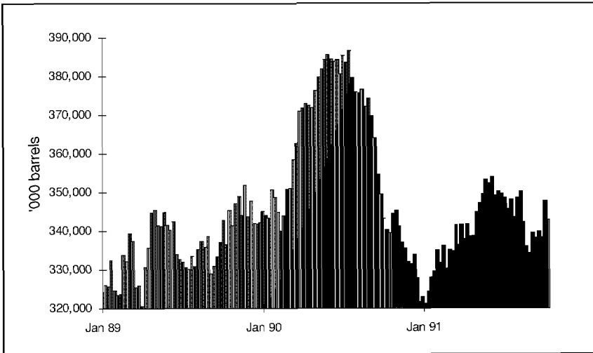
Figure 11.7 US crude oil stocks, end-week
