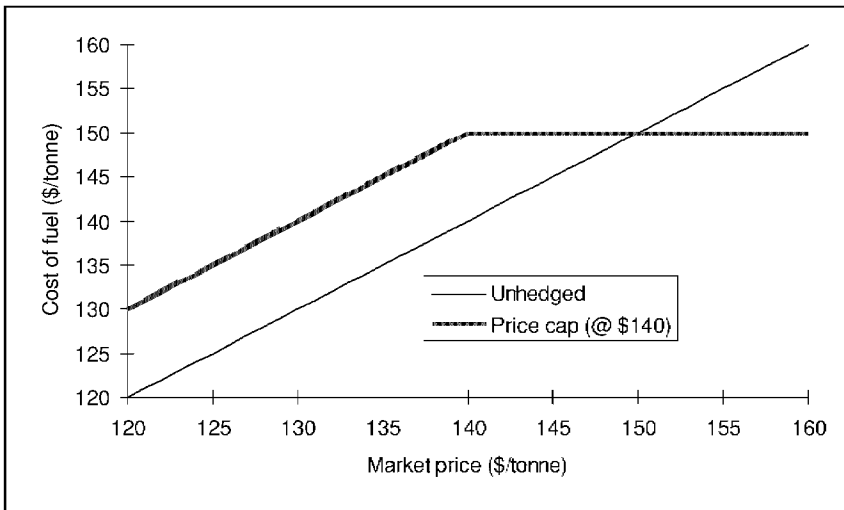
Figure 10.10 Result of hedging using a price cap
