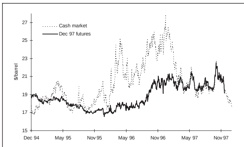
Figure 6.2 Convergence of WTI futures and cash markets
