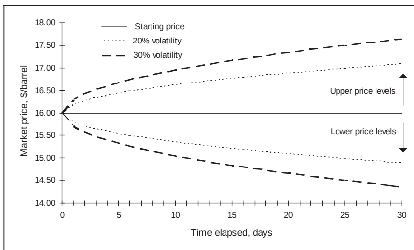
Figure 9.21 Effect of volatility on market trading range
