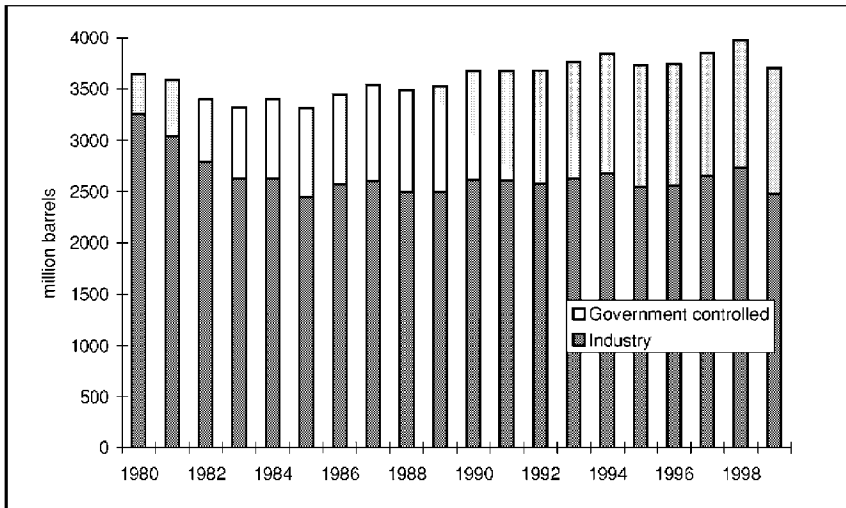
Figure 1.4 Total stocks held in OECD countries, end year
