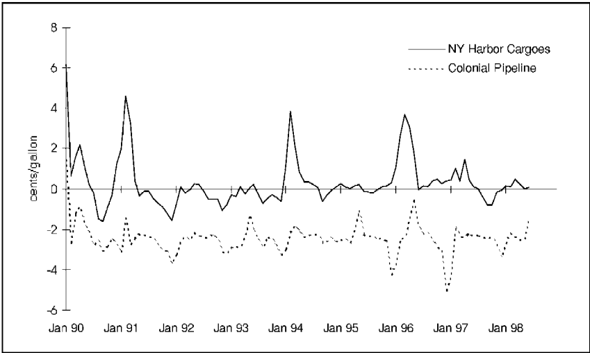
Figure 5.11 Distillate fuel oil: spot minus Nymex futures prices
