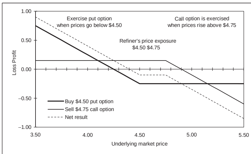
Figure 9.15 Hedging refinery margins, low cost collar option
